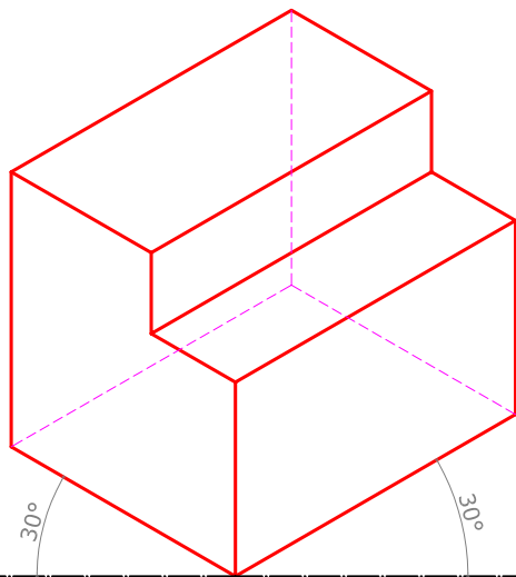
ISOMETRIA 30° - 30°
